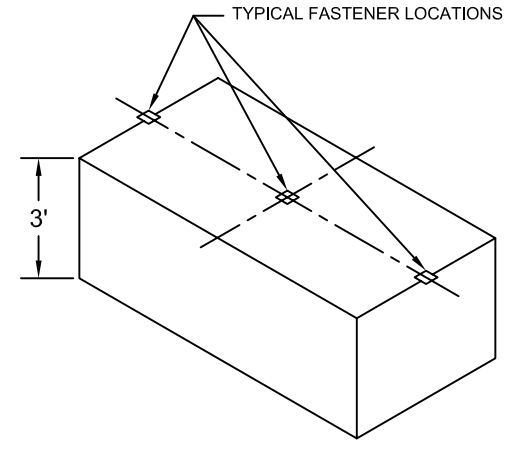
TYPICAL GEOFOAM BLOCK
