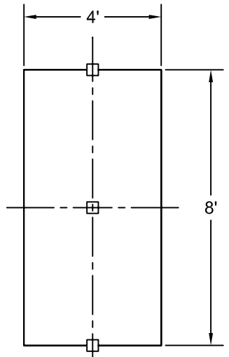
TYPICAL GEOFOAM BLOCK
